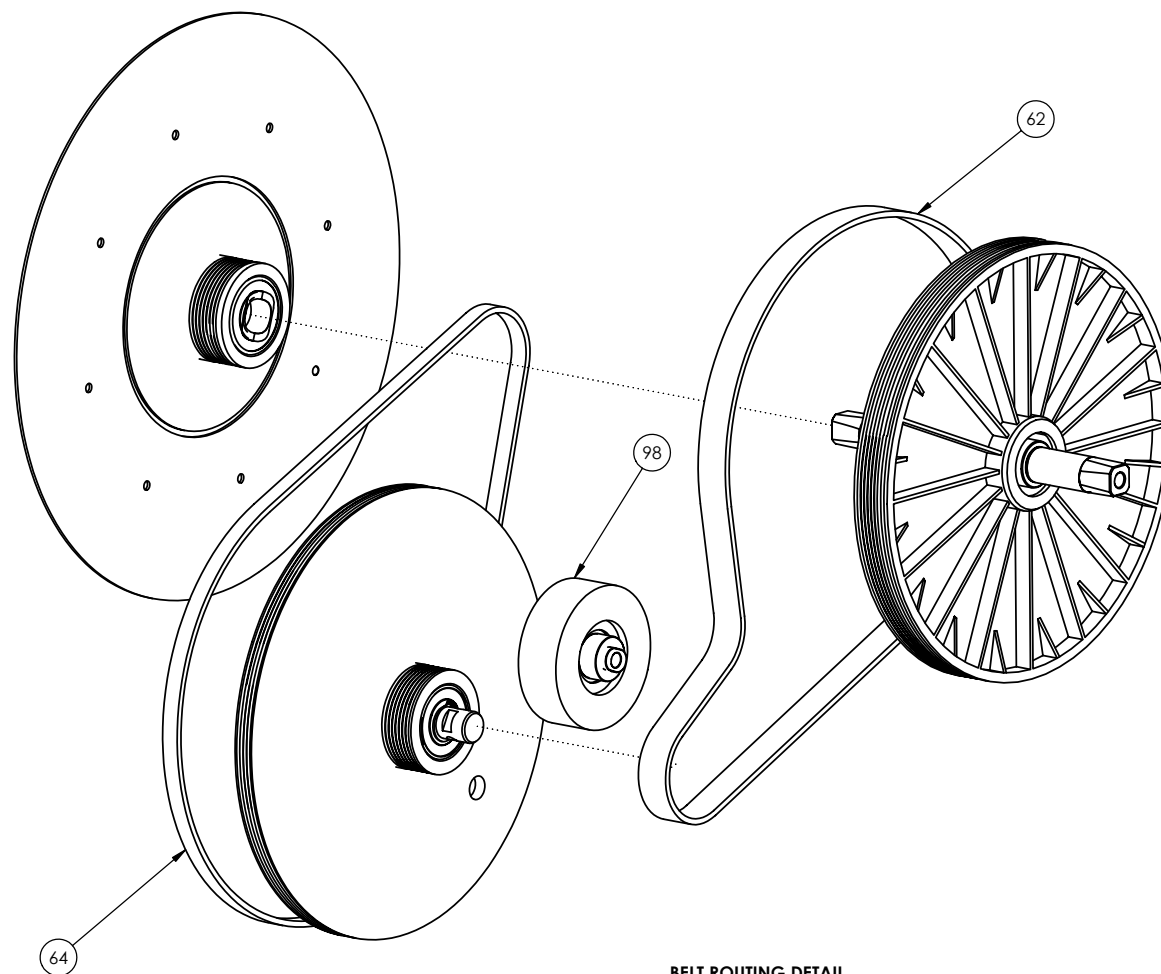
BELT ROUTING DETAIL
